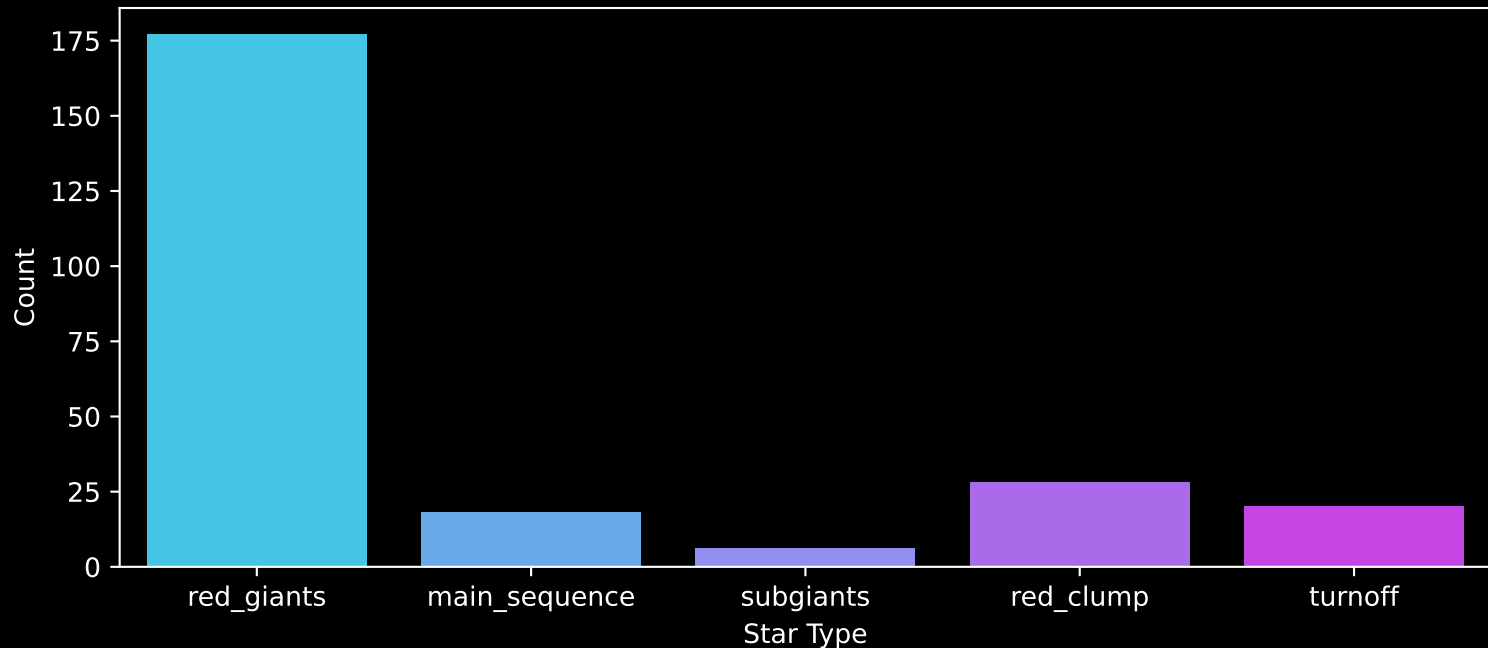
APOGEE DR17 Field: [034+12] Count plot of Star Type
