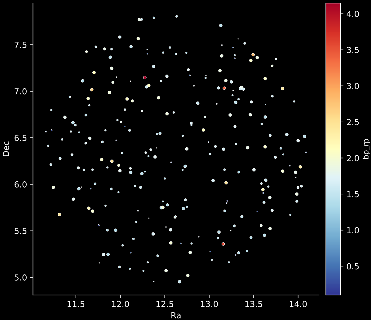
APOGEE DR17 Field: [034+12] Stars: 249
