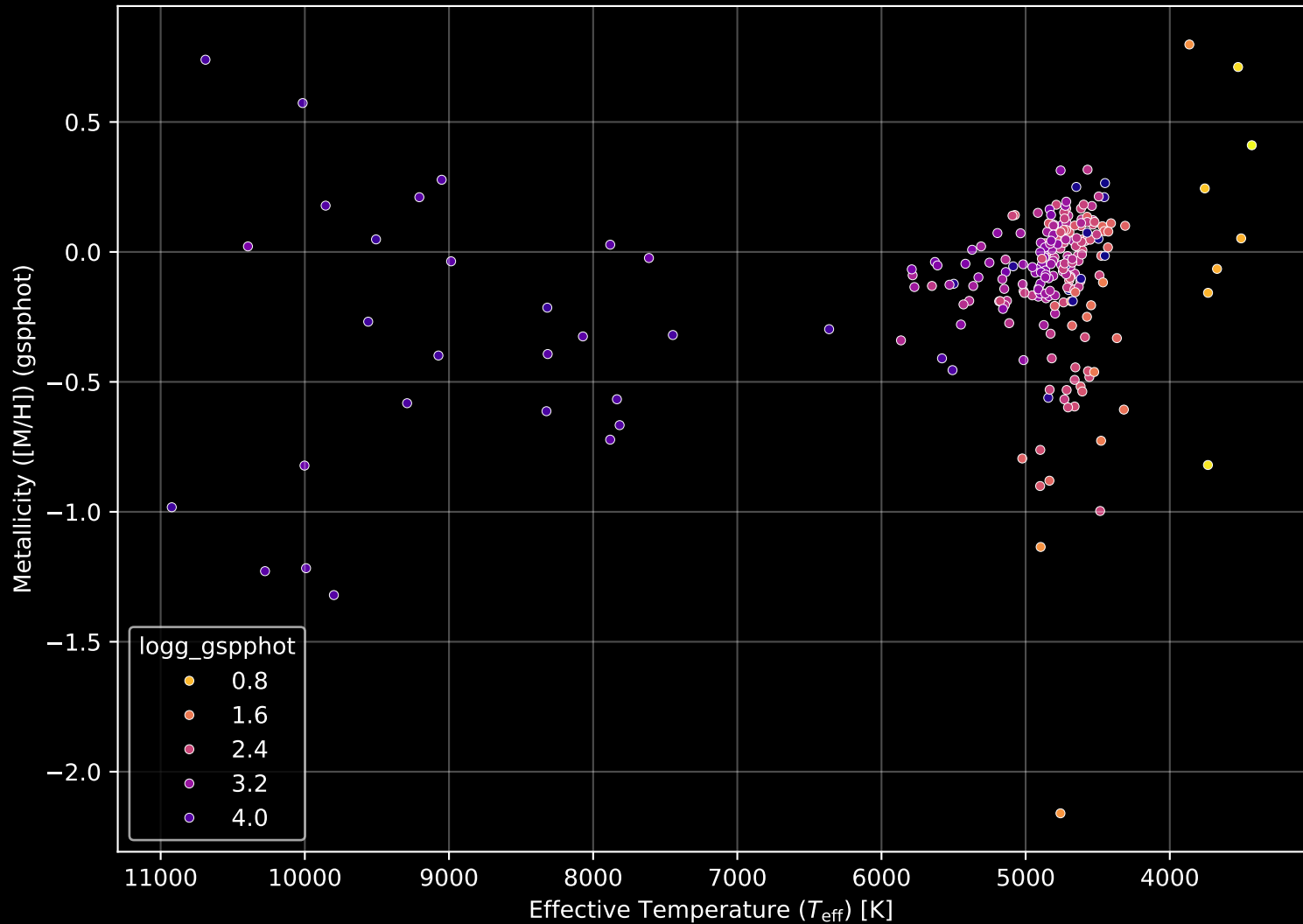
APOGEE DR17 Field: [034+12] Stellar Population Parameters (n= 249)
