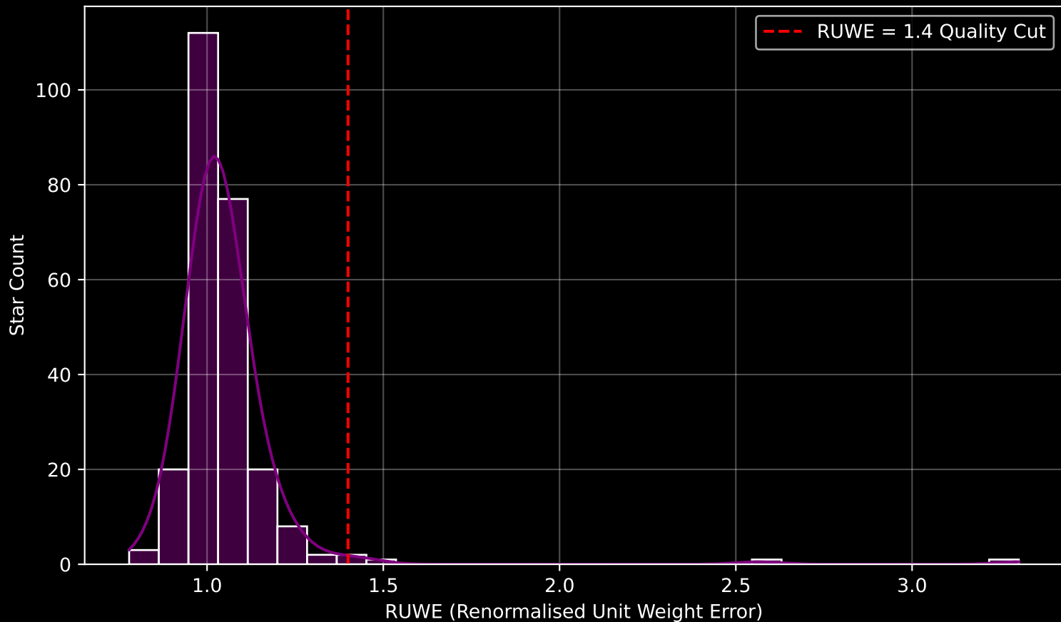
GAPOGEE DR17 Field [034+12] RUWE Distribution (n= 247)
