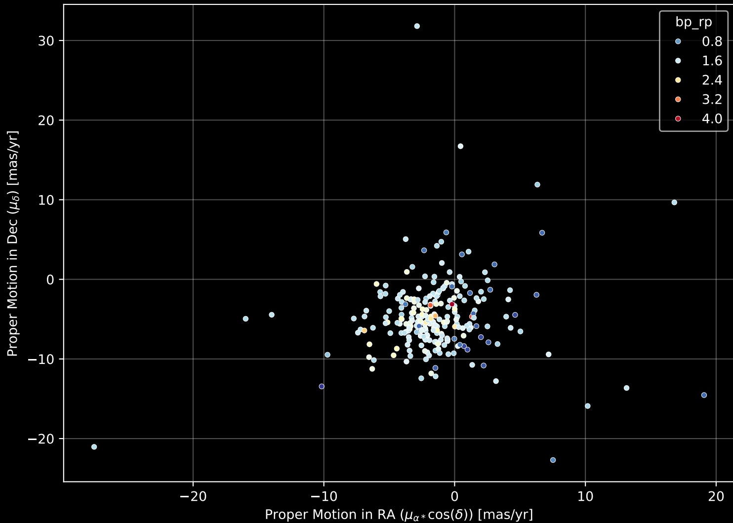
APOGEE DR17 Field: [034+12] Proper Motion Diagram (n= 249)
