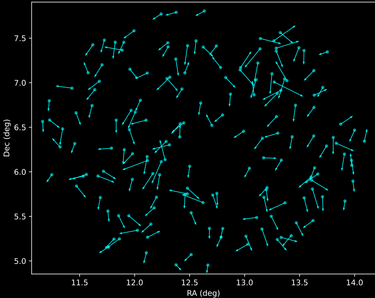
APOGEE DR17 Noise Stream Proper Motion Vectors (n=161)
