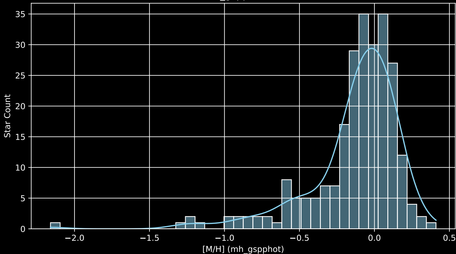
APOGEE DR17 Field: [034+12 [M/H] (mh_gspphot) (n= 245)
