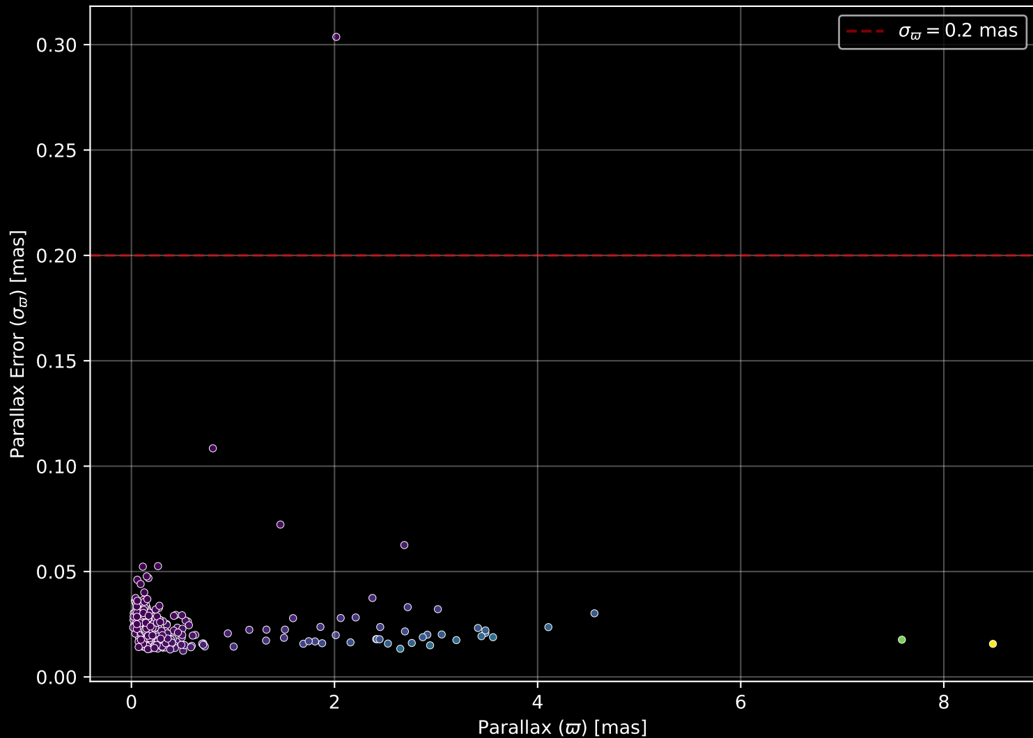
APOGEE DR17 Field: [034+12] Parallax Quality (n= 249)
