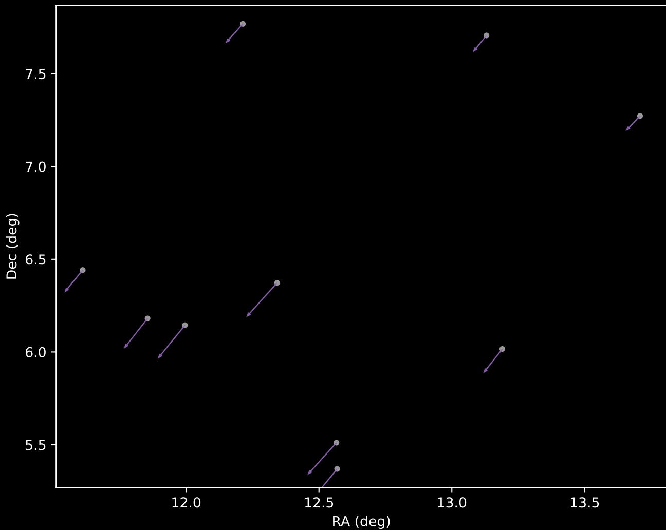
APOGEE DR17 Cluster 8 Proper Motion Vectors (n=10)
